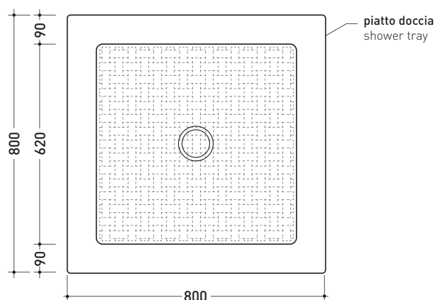
piletta ø 90 (in dotazione) drain ø 90 (included in the box)
