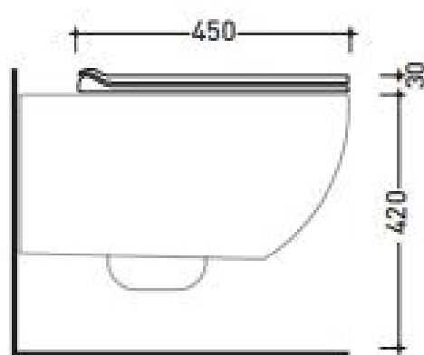
art. AP118 - AP118G vista laterale / lateral view
