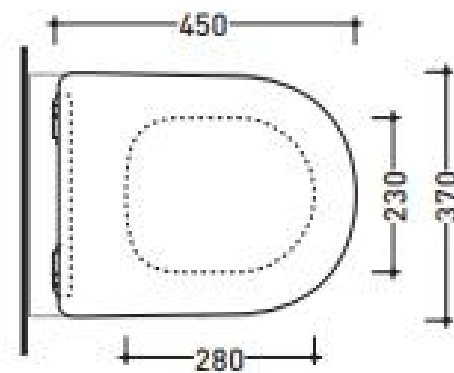
art. AP119 - AP119G vista zenitale / zenital view
