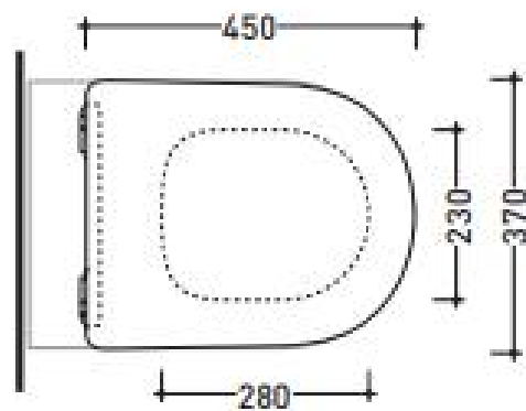
art. AP117G - AP117RG vista zenitale / zenital view
