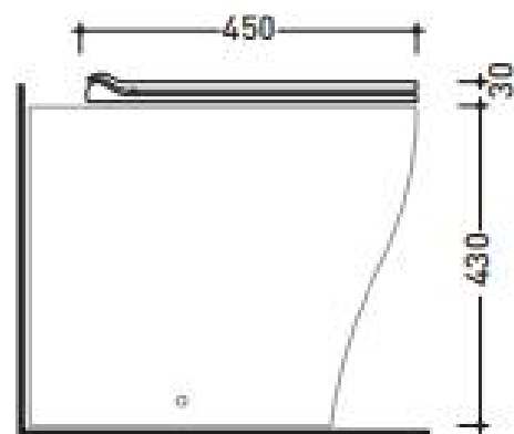
art. AP117G - AP117RG vista laterale / lateral view
