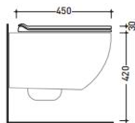
art. AP119 - AP119G vista laterale / lateral view
