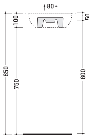
vista retro / back view
