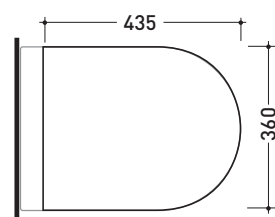
art. 5064 vista zenitale / zenital view
