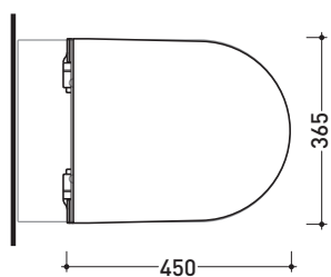
art. AP118 vista zenitale / zenital view
