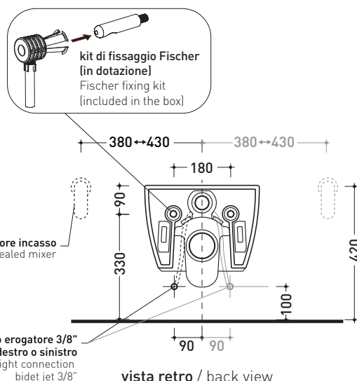
vista retro / back view
